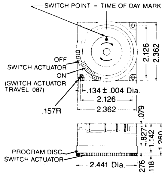
Figure 1 — Dimensions
